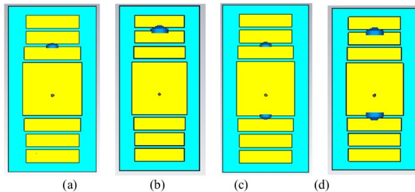
Figure 3. The position of PIN diode in patch antenna
