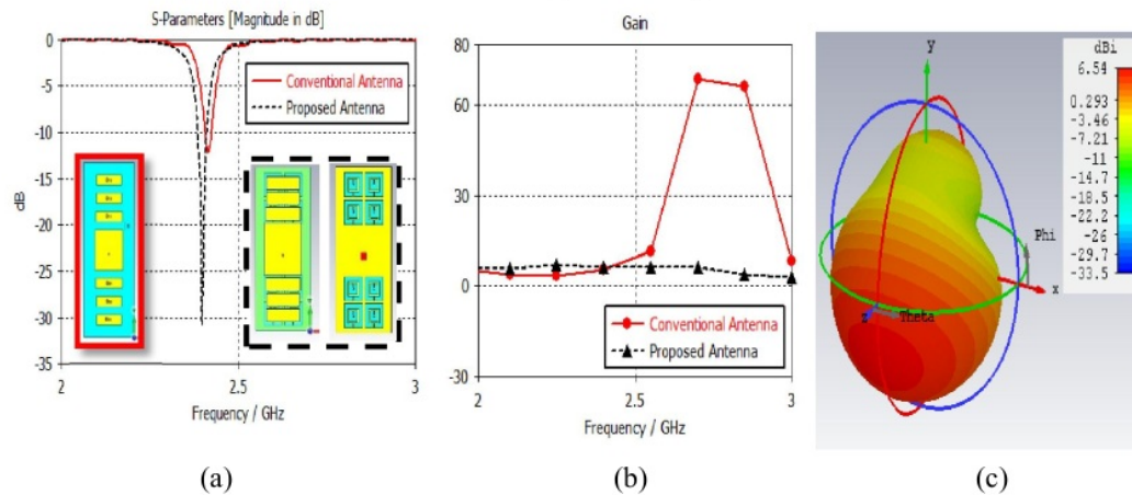
Figure 2. Proposed antenna performance (a) S-Parameter Compared, (b) Gain Compared dan (c) Radiation Pattern 2.4 GHz
